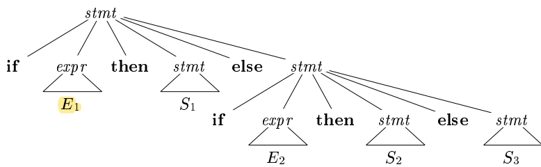
Figure 4.8: Parse tree for a conditional statement
