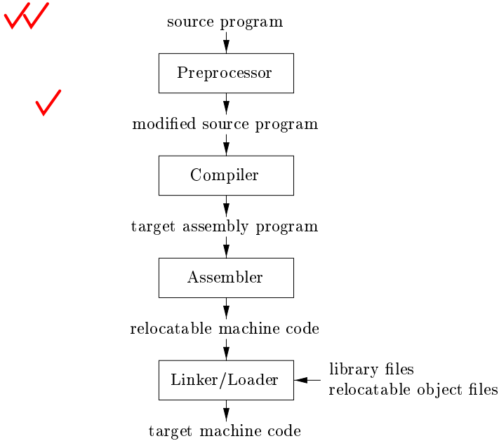
Figure 1.5: A language-processing system
