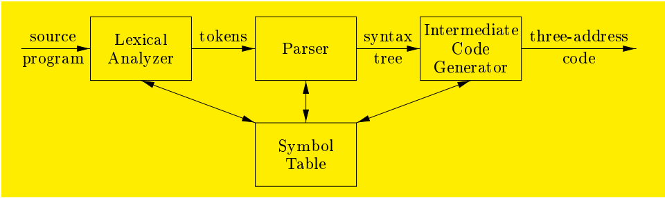
Figure 2.3: A model of a compiler front end
