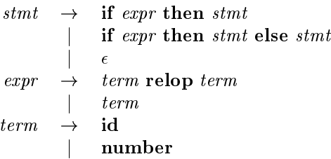
Figure 3.10: A grammar for branching statements
