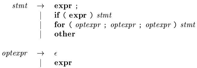
Figure 2.16: A grammar for some statements in C and Java
